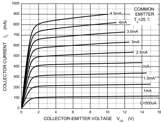
Static Characteristic
